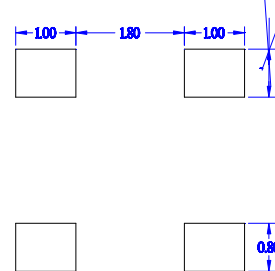
Recommended stencil size
